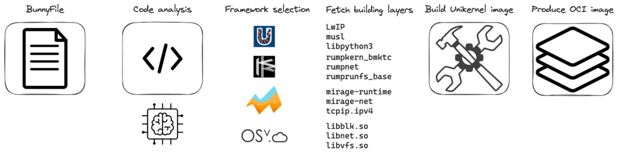
Figure 13: High-level overview of the Bunny workflow
