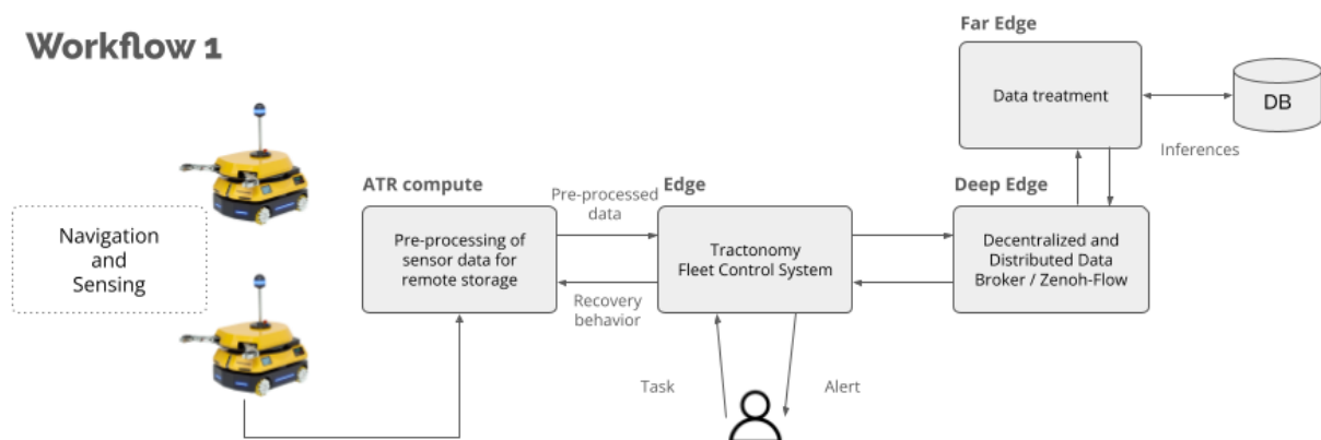
Figure 27: UC3 preliminary deployment view – 1 st workflow
