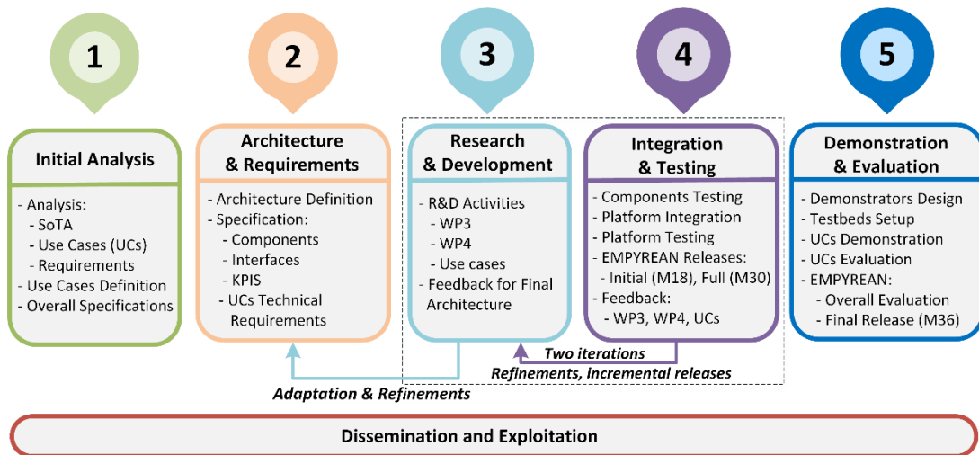
Figure 31: Overall technical development strategy and methodology
