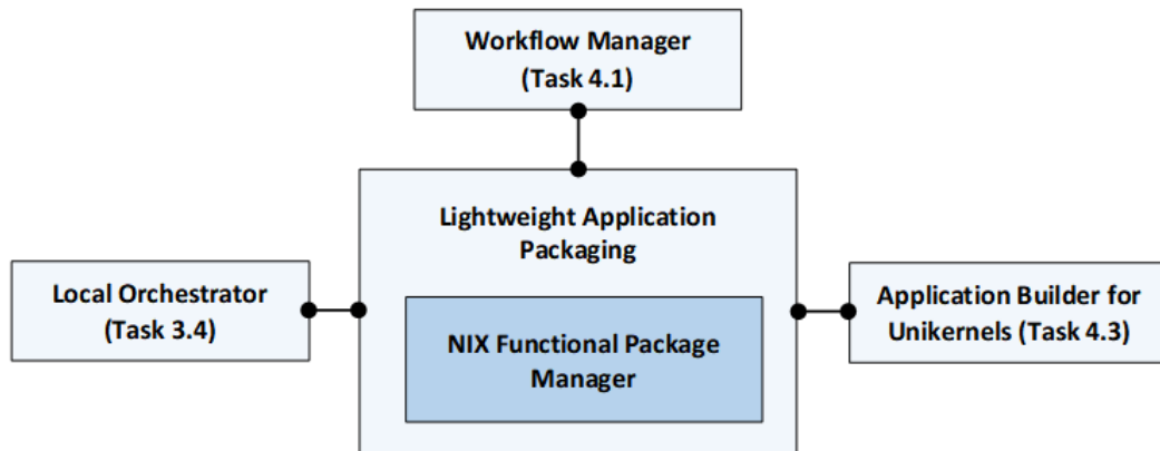
Figure 12: NIX-based Environment Packaging components and dependencies
