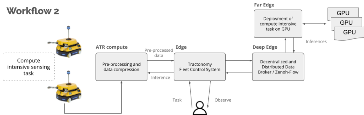
Figure 28: UC3 preliminary deployment view – 2 nd workflow
