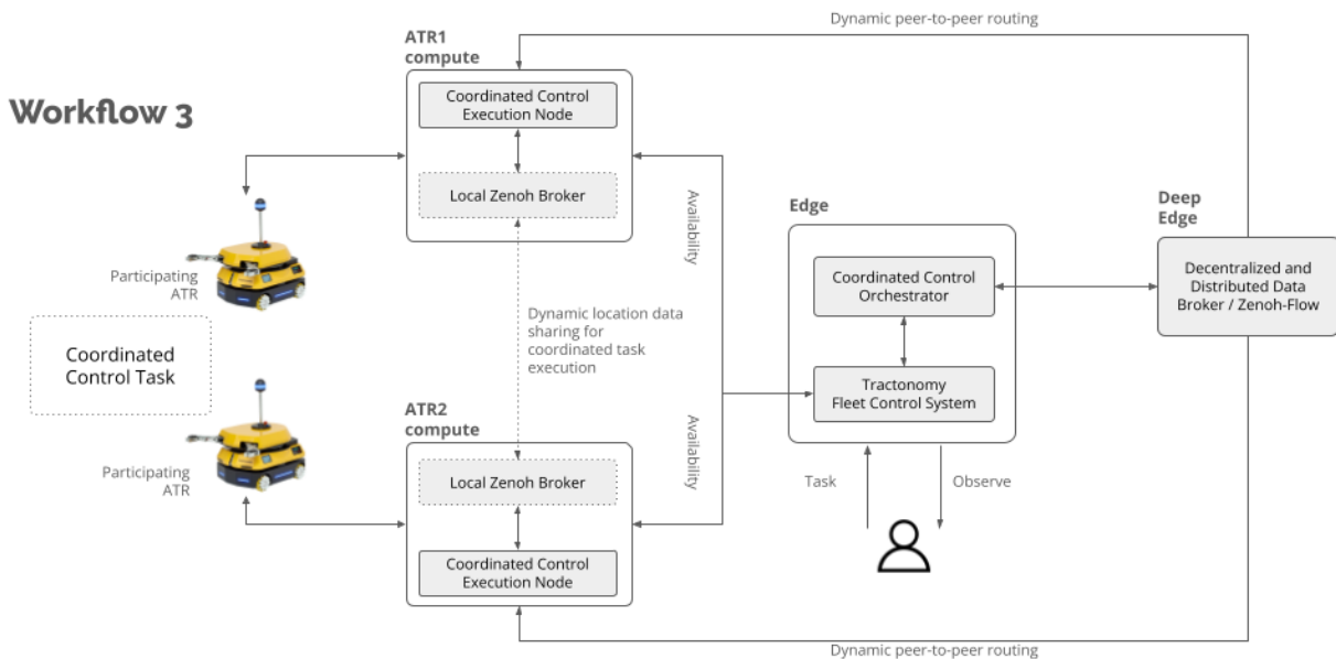
Figure 29: UC3 preliminary deployment view – 3 rd workflow
