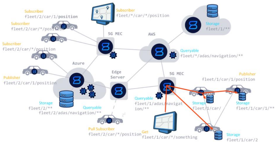
Figure 5: Distributed data query in automotive context
