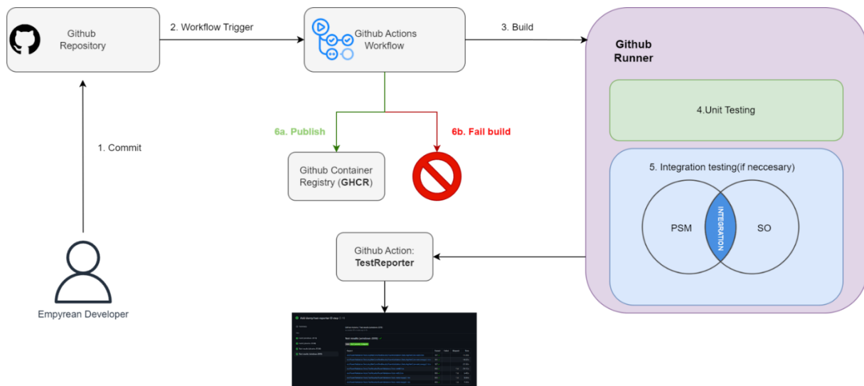
Figure 30: CI/CD workflow
